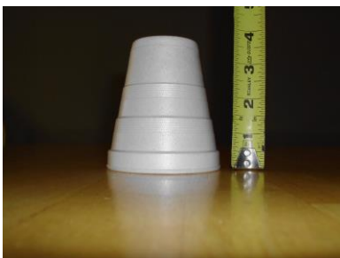
20 – Styrofoam cup “canal supports” 3 3/4" high. When stacked, each cup adds an additional 1/2" of height.
